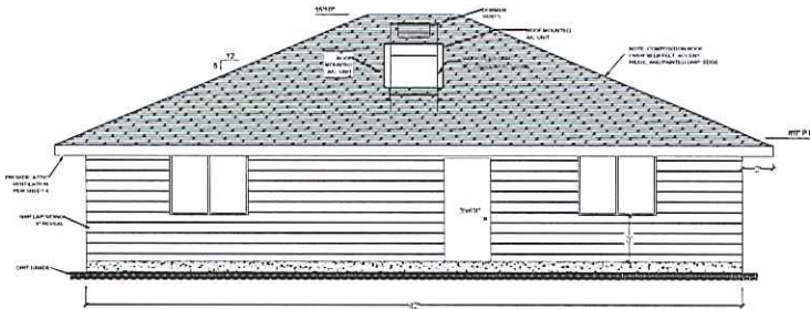
SOUTH ELEVATION
