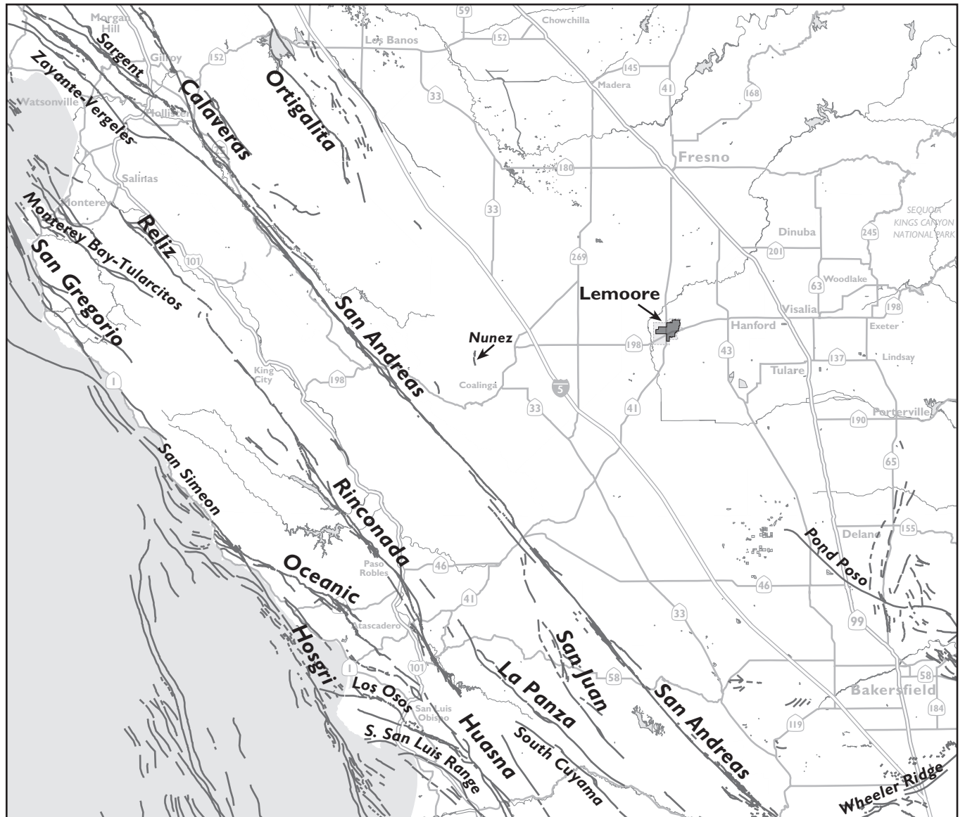
Figure 8-1 Regional Faults
