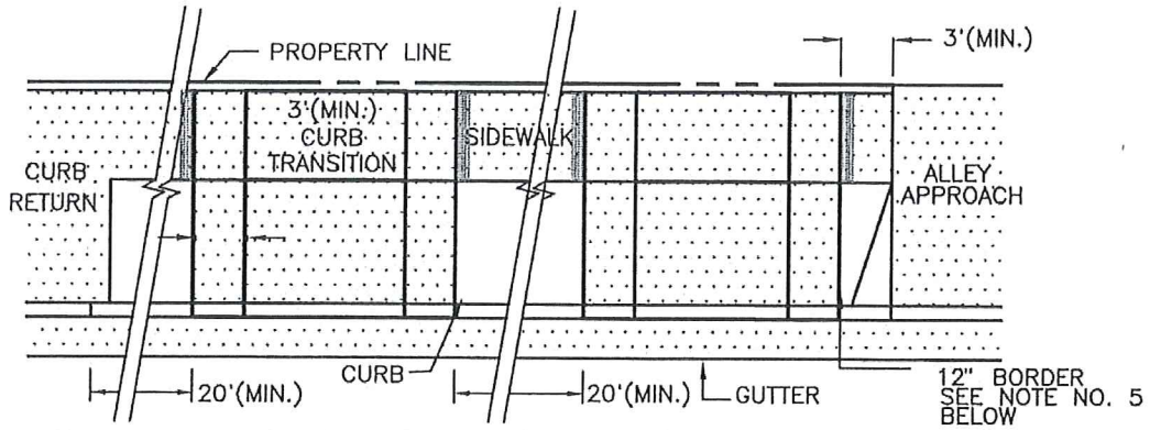
DRIVE APPROACH WITH NON-CONTIGUOUS SIDEWALK
